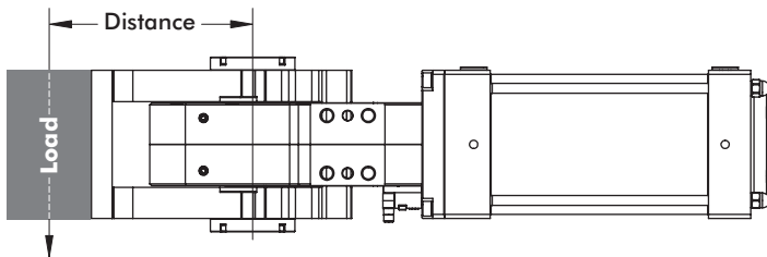
Max. applicable load with swivel unit positioned on its side (6 bar [87 psi])
